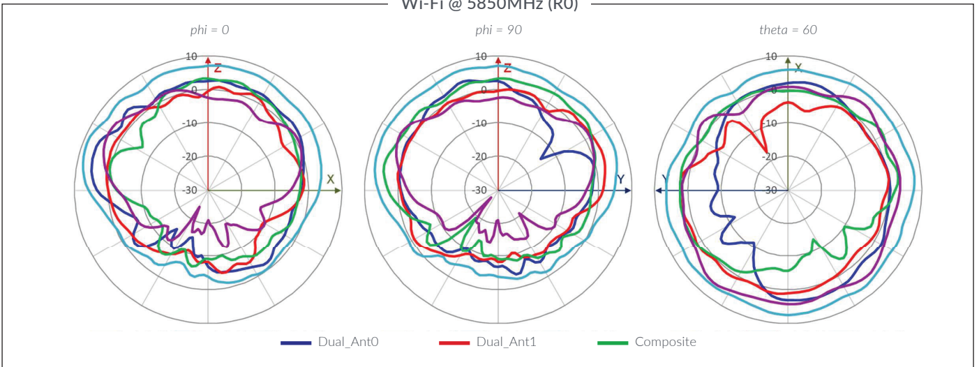
Wi-Fi @ 5850MHz (R0)
